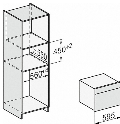
H 7 x 40BM/BMX, schets
