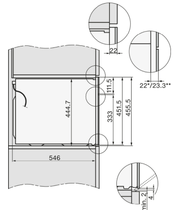
H 7 x 40 BM/BMX, schets, GB, AUS
