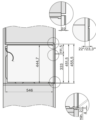
H 7 x 40BM/BMX, schets
